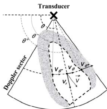
Fig. 1. Sketch of an echocardiographic acquisition in the apical long-axis view. The dashed outline delimits the plane of interest corresponding to the LV cavity. \vec{V} represents the velocity of a given blood particle, V_r is its radial component measured by color-Doppler and V_\theta the azimuthal component to be determined using the continuity equation. V_{\theta^-} and V_{\theta^+} are the azimuthal velocities at the posterior and anteroseptum walls (equation 2), respectively.
