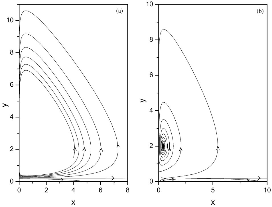
Fig. 4. Phase portraits (lymphocytes population versus malignant cells). (a) \alpha = 2, k = 0.2 and \sigma = 0.09 . (b) \alpha = 2, k = 0.2 and \sigma = 0.25 .
